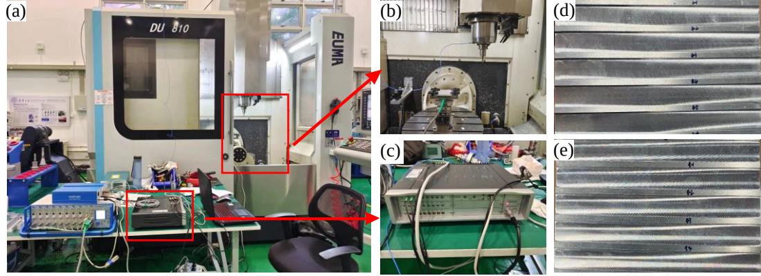
Figure 6: Experimental equipment and data analysis illustration
