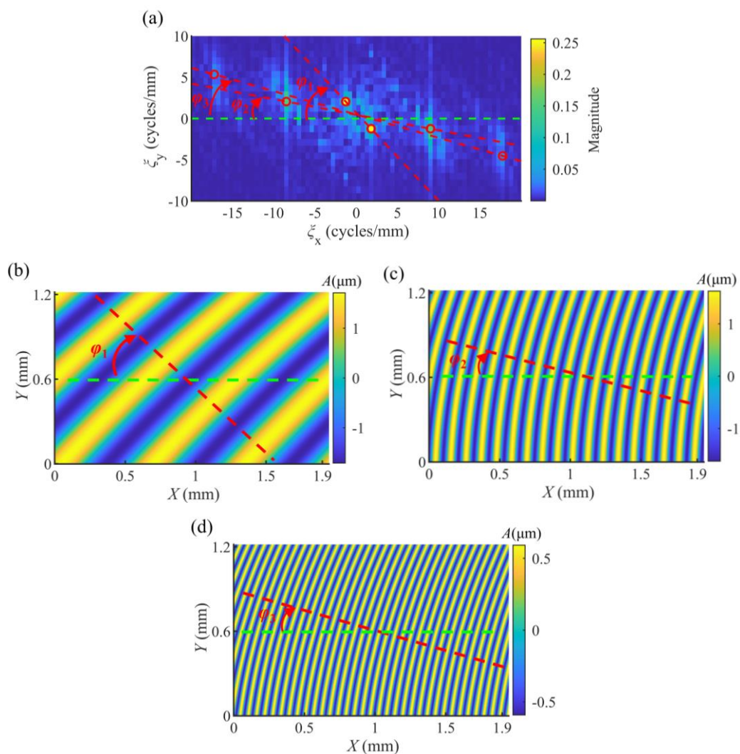
Figure 3: Superposition angle identification from 2D FFT spectrum
