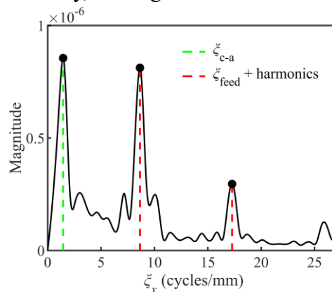
Figure 2: Dominant amplitude and spatial frequency identification from FFT spectrum
