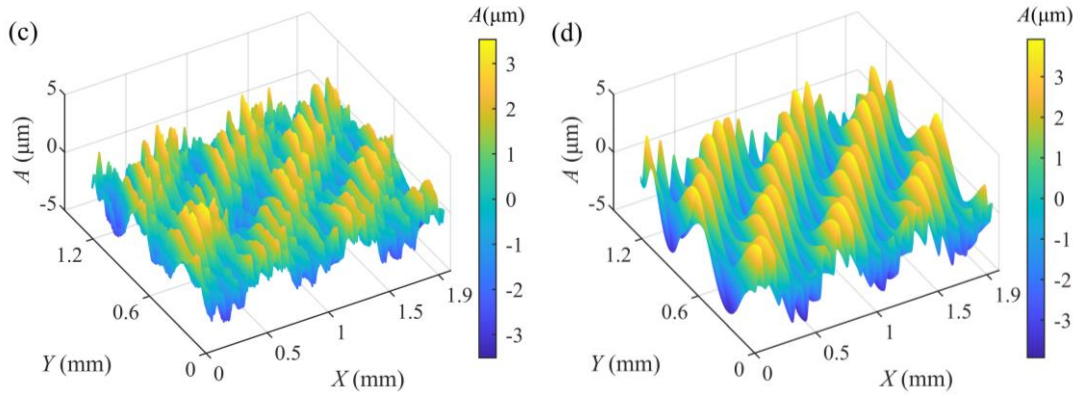
Figure 4: Superposition of three dominant marks (a) Scanned 2D surface; (b) Reconstructed 2D surface; (c) Scanned 3D surface; (d) Reconstructed 3D surface
